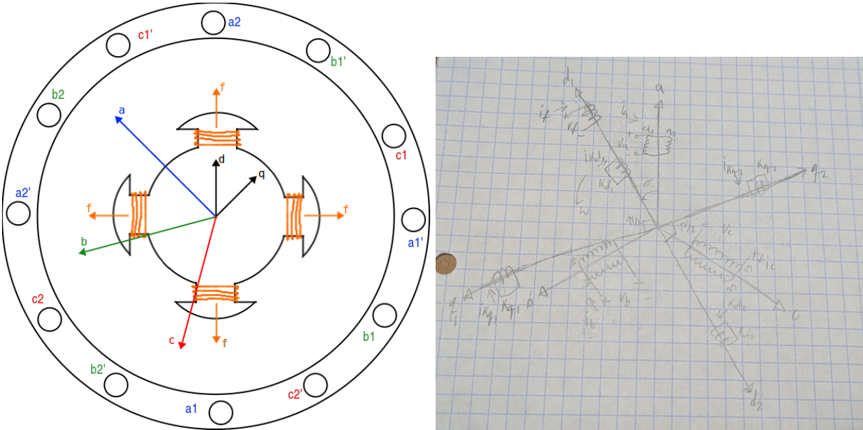
Fig. 1. Cross-section of generator, not to scale. The quadrature (q) axis is 90° electrically from the direct (d) axis. Because this is a 4-pole generator, there are 720° electrical for every 360° mechanical. The analysis would be the same if a, b, c, d, and q were rotated a multiple of 90° mechanical (180° electrical).
